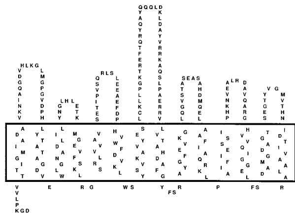
FIG. 3. Proposed topology of Tromp1. Sequences within the rectangle indicate 14 membrane-spanning regions having amphipathic beta-sheet structures. Sequences above the rectangle indicate seven surface-exposed loops. Sequences below the rectangle indicate regions exposed to the periplasmic space.
